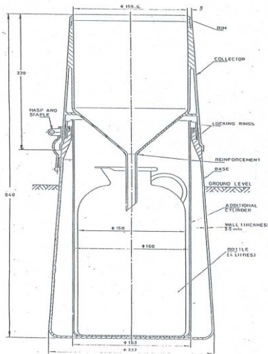
Fig 11 Rain Gauge, Non-Recording (200 cm 2 ), General Assembly
