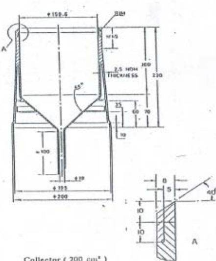
Collector (200 cm 2 )
